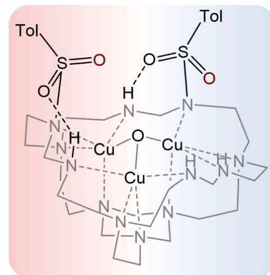
O 2 activation
