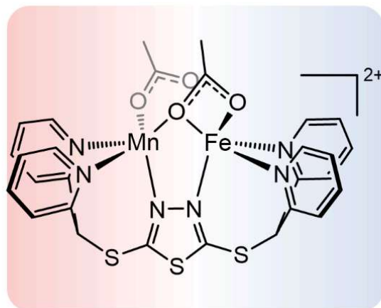
Heterobimetallic selectivity
